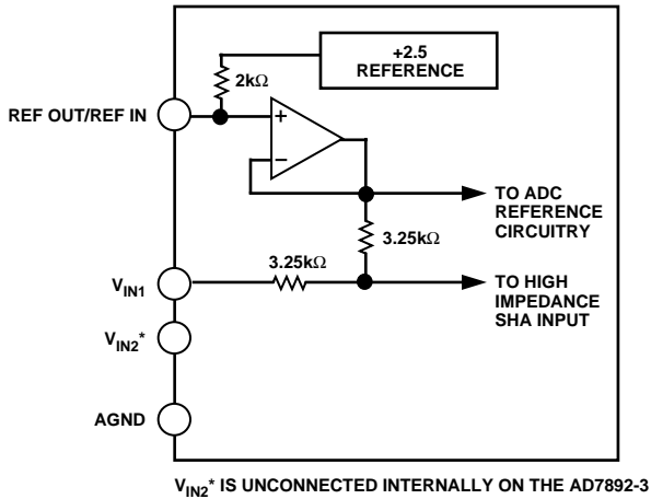
Figure 5. AD7892-3 Analog Input Structure
