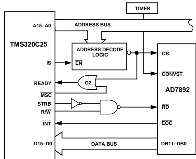
Figure 7. AD7892 to TMS320C25 Interface
