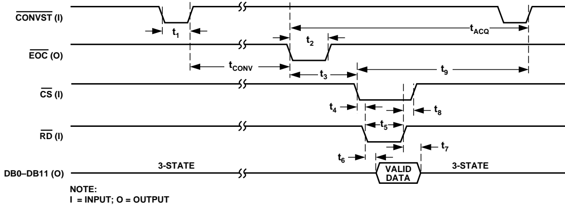
Figure 2. Parallel Mode Timing Diagram
