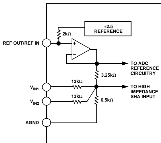
Figure 4. AD7892-1 Analog Input Structure
